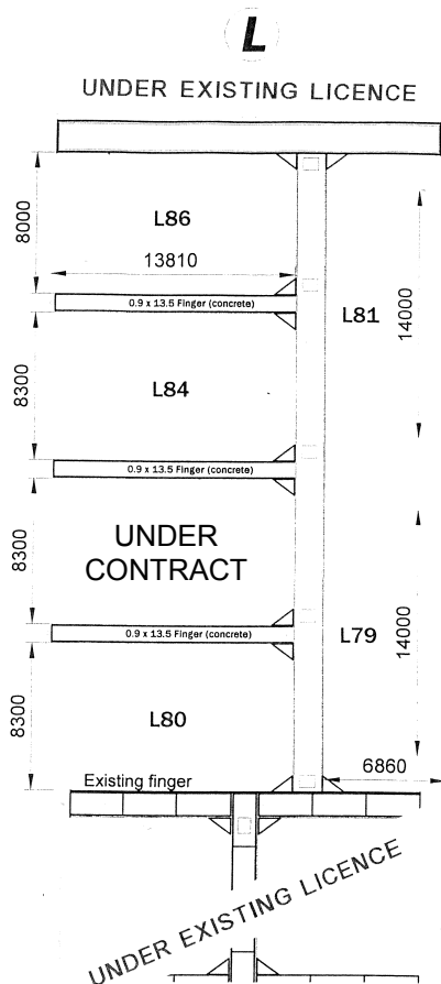
PROPOSED RECONFIGURATION PLAN LAYOUT SCALE 1:250
